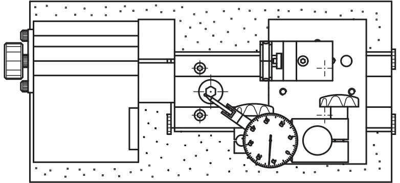
Example with support prism for long parts
