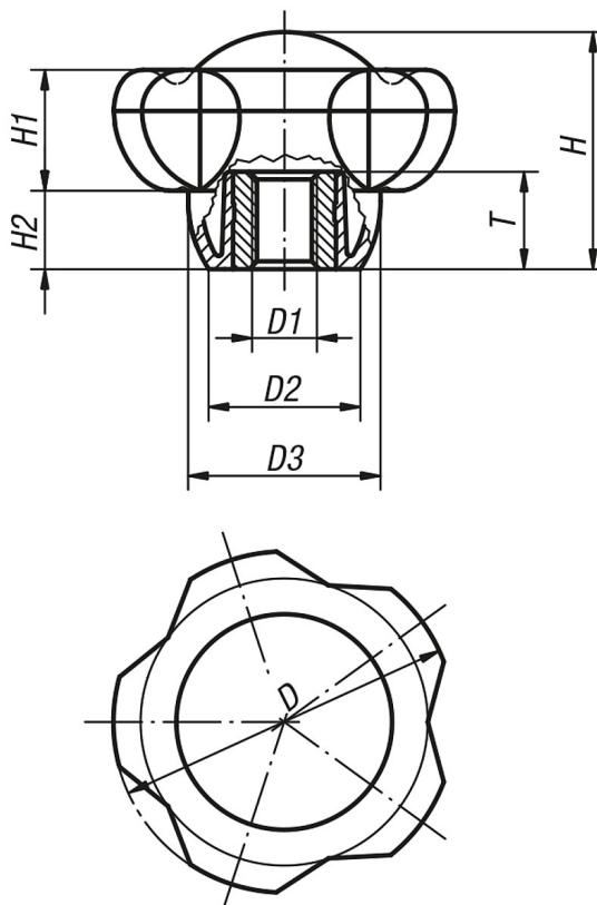
Clamp Grip with internal thread
