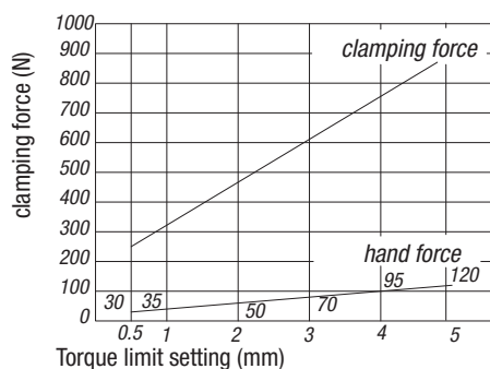
Pull Clamps 04400-3240...
