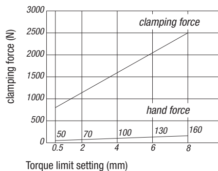
Pull Clamps 04400-4050...
